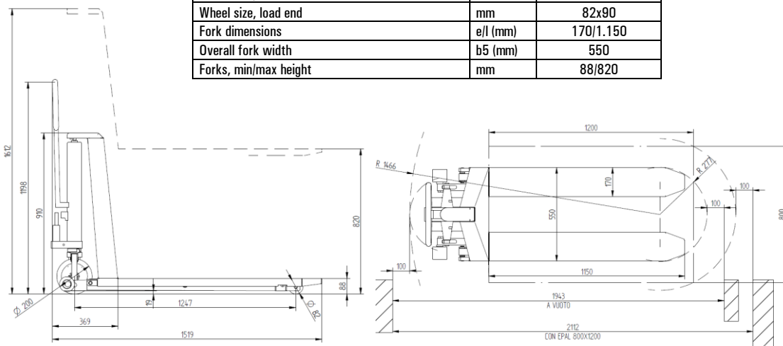
Lateral axles for maximum stability
